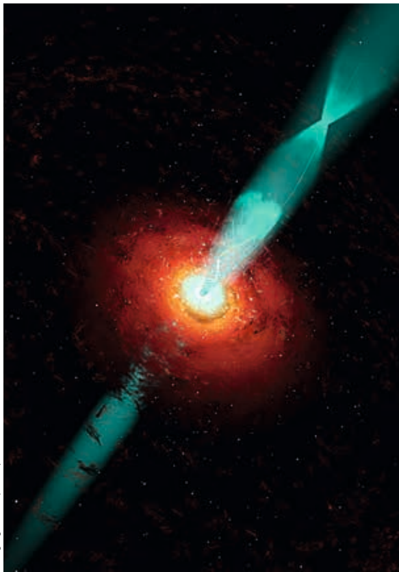
Figura 3. Still from a conceptual animation of 3C 120 created by Wolfgang Steffen. A bipolar outflow of relativistic particles is produced by the super massive black hole at the centre of an active galaxy.
